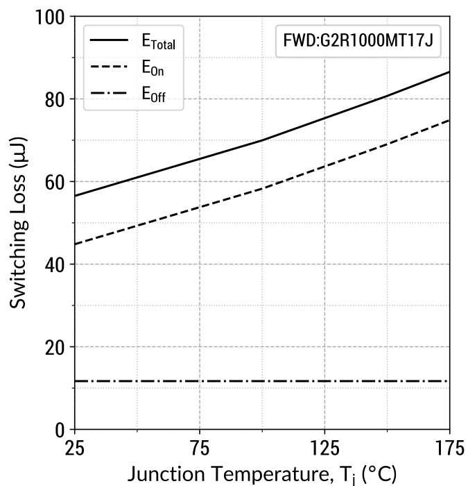
Figure 25: Inductive Switching Energy v/s Temperature ( V_{DD} = 1200V )
