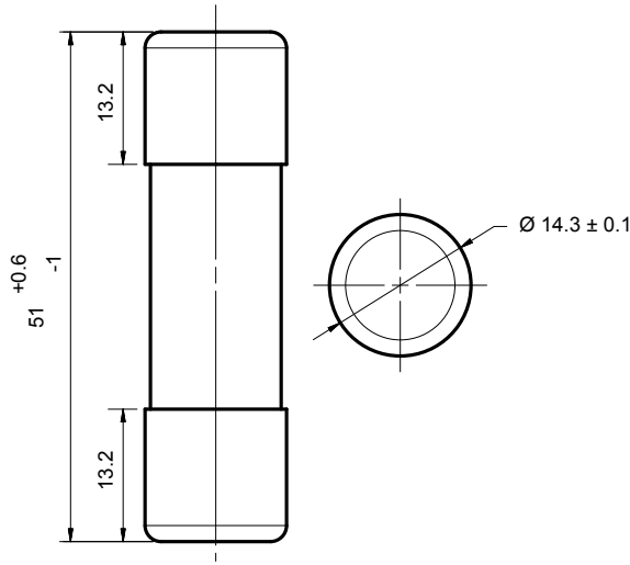
CP 14x51 gR without striker (100212)
