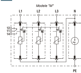
G 3+1 (4PG)
