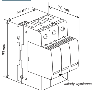
3 poles
