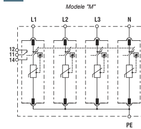
H 4+0 (4P)
