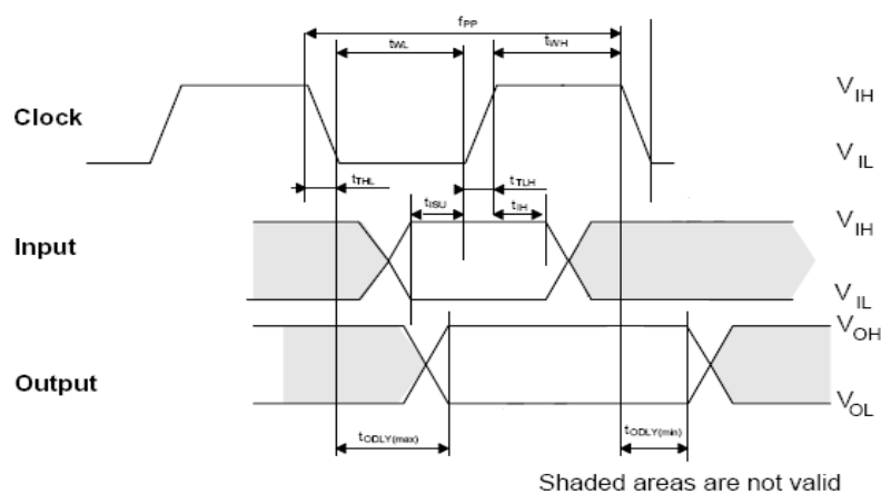
Figure 3 – Input/Output Timing (Default Speed Mode)
