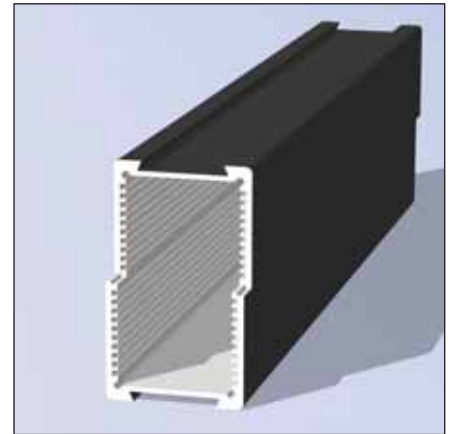
Two half-shell extrusions with integrated guide rails for 42 mm PC boards and exterior slots designed for optional 35 mm DIN Rail mounting bracket.
