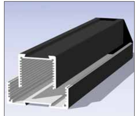
Two half-shell extrusions with integrated guide rails for 42 and 72 mm PC boards and exterior slots designed for optional 35 mm DIN Rail mounting bracket.
