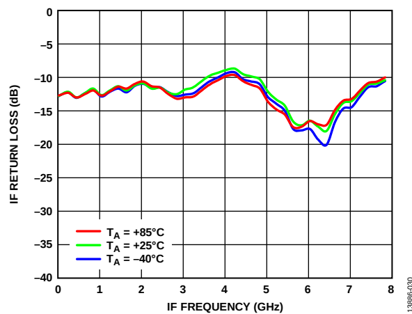
Figure 30. IF Return Loss vs. IF Frequency at Various Temperatures, LO = 25 GHz, 13 dBm
