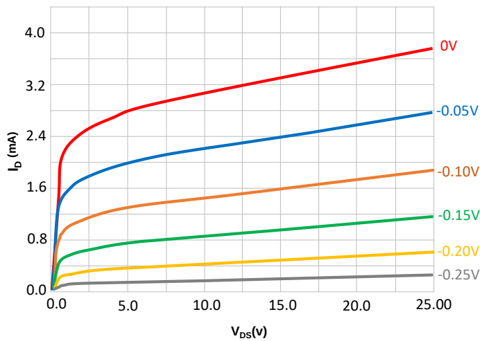
Figure 9. I_D vs. V_{DS} vs. V_{GS}
