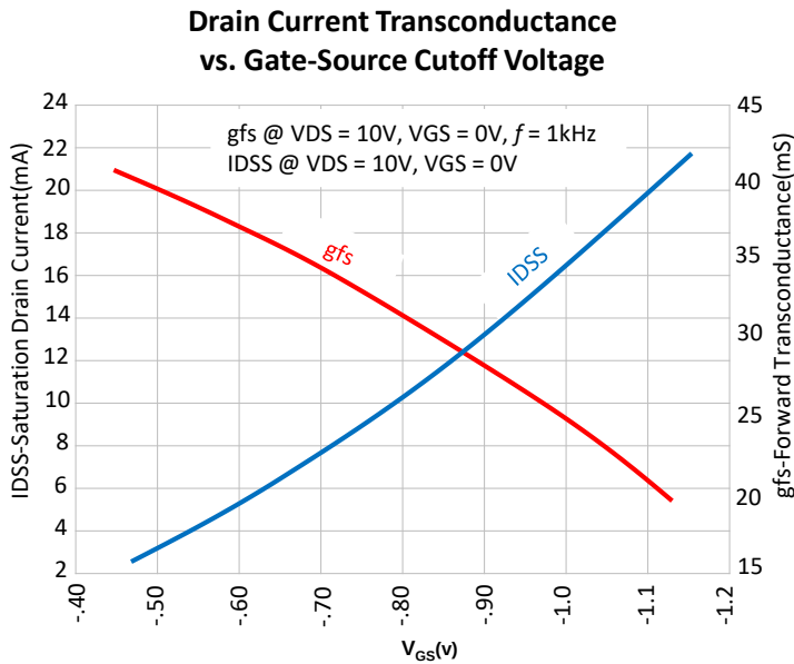
Figure 21. V_{GS} (cutoff) vs. I_{DSS} vs. G_{FS}
