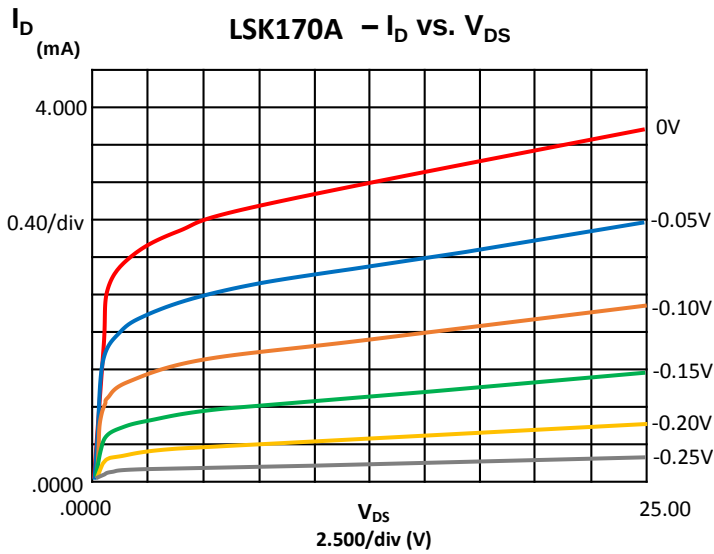
Output Characteristics
