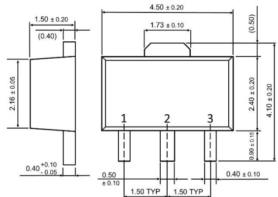
SOT-89 3 Lead
