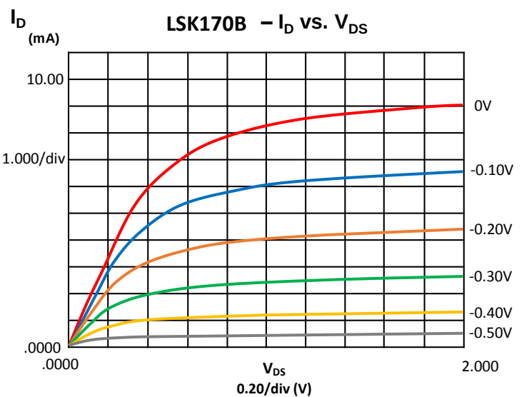
Operating Characteristics
