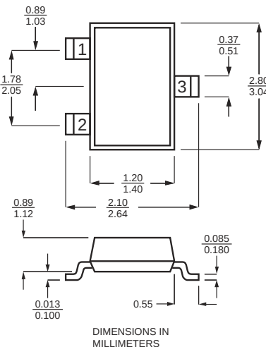
SOT-23 3 Lead
