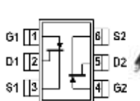
SOT-23 6L Top View
