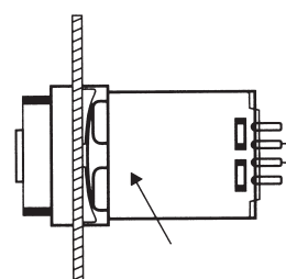
PANEL MOUNTING BRACKET ATC P/N 406-320-02-00
