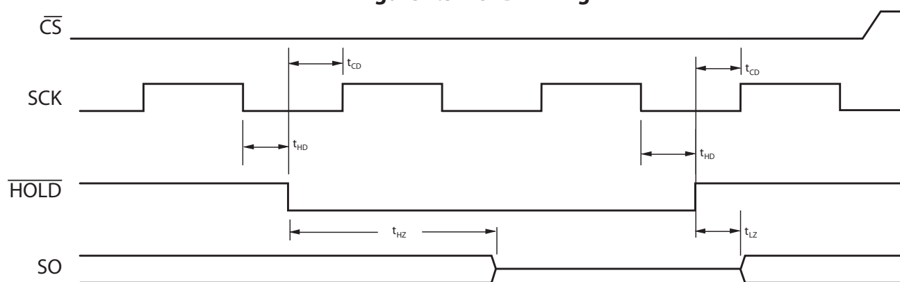
Figure 4.5 HOLD Timing
