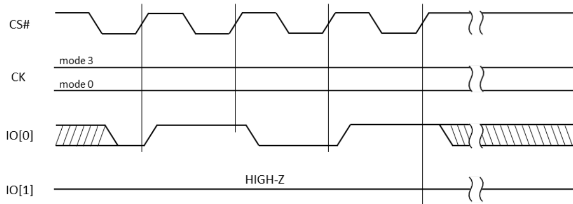
Figure 37 Reset with Signal Sequence (JEDEC 252)
