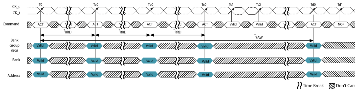
Figure 33 - tFAW Timing
