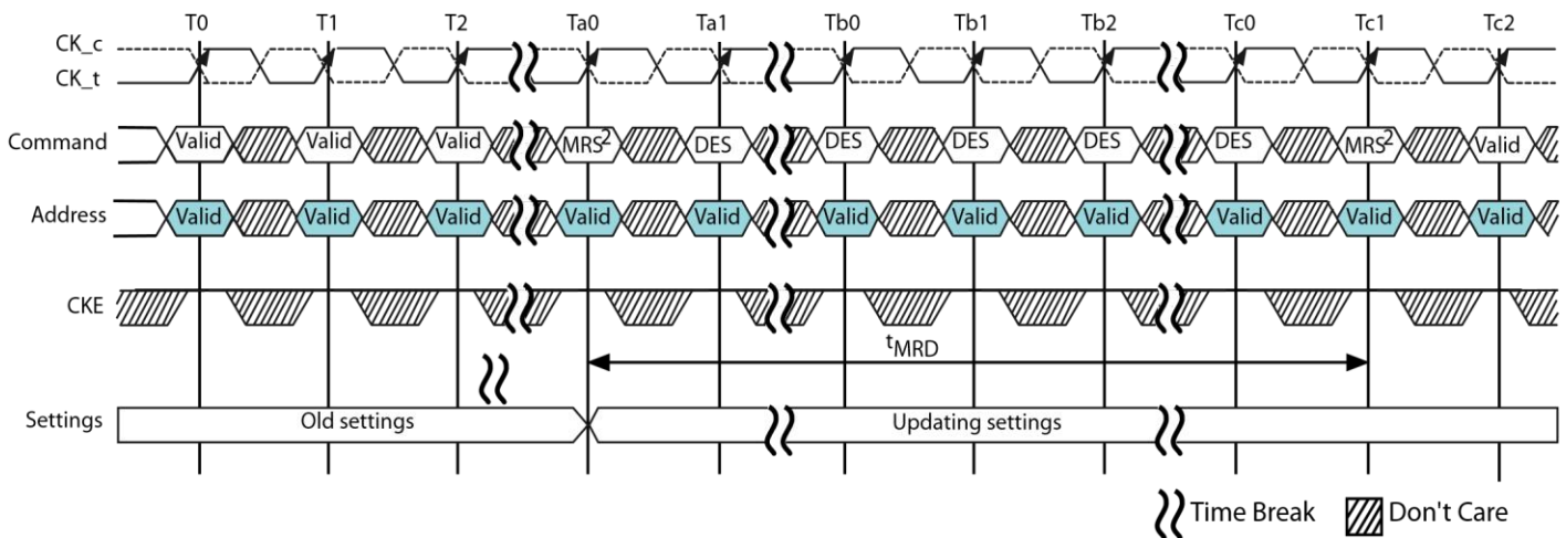
Figure 7 - t MRD Timing
