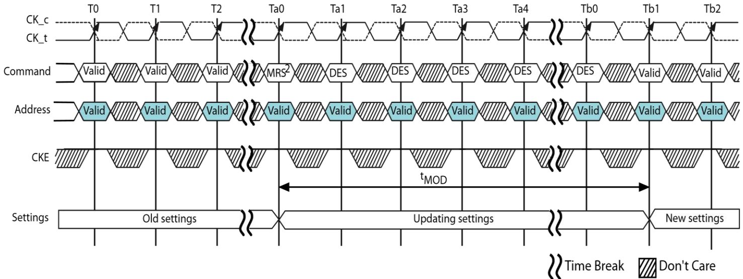
Figure 8 - t_{MOD} Timing
