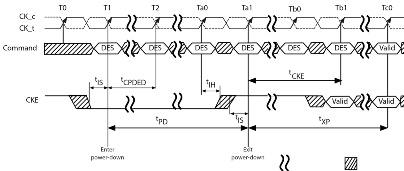
Figure 40 - Precharge Power-Down Entry and Exit
