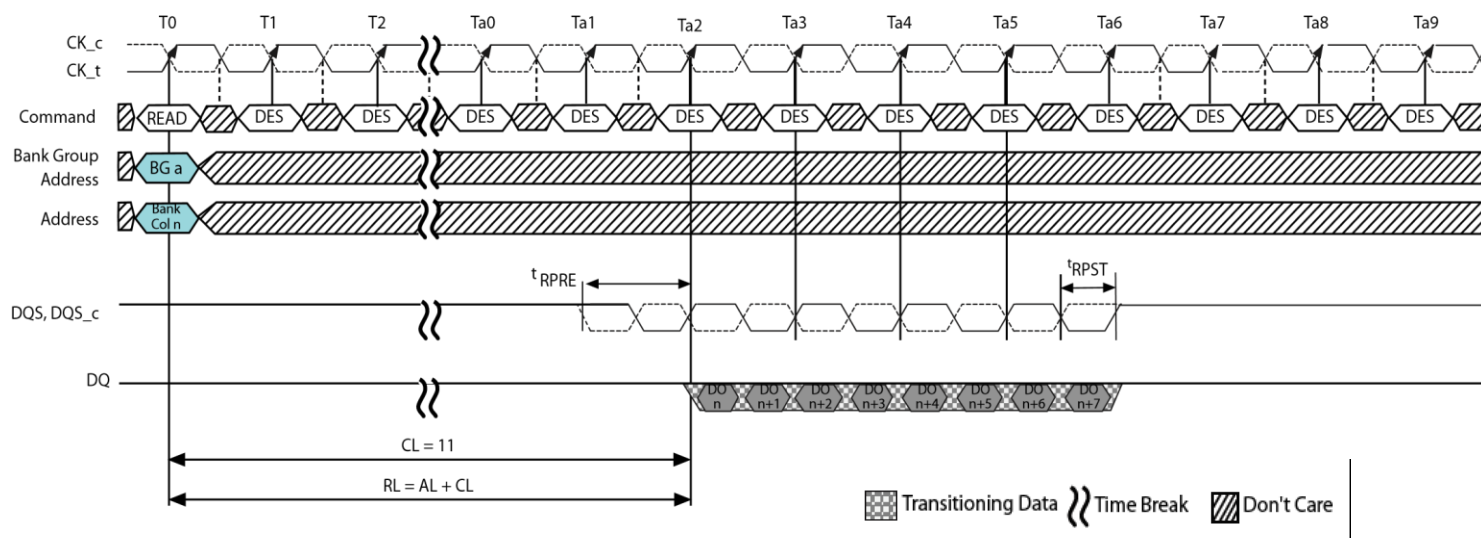
Figure 52 - READ Burst Operation, RL = 10 (CL = 10, BL8)
