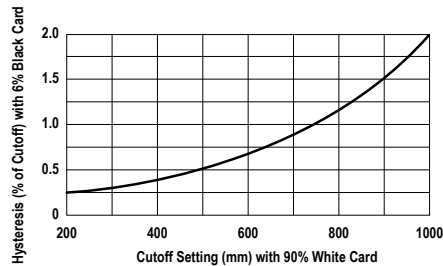
Figure 11. Hysteresis
