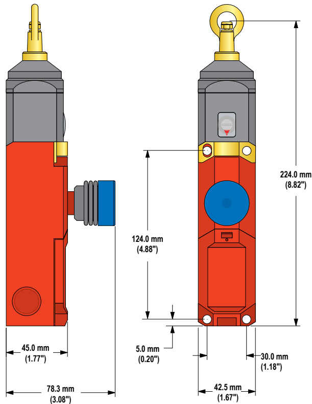
Figure 14. RP-LS42F..L Models
