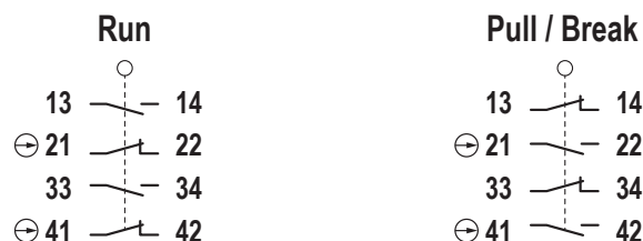
Figure 1. Contact State
