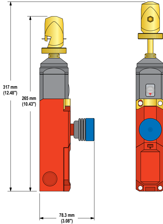
Figure 15. RP-LS42F-xxLF Models
