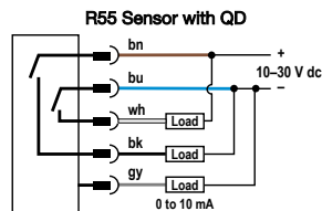
R55 Sensor with 5-pin Euro-style QD
