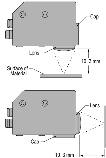
Figure 4. Mounting Distance and Lens Positions
