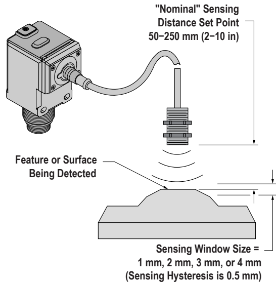
Figure 3. Sensing Distance Set Point and Window Size
