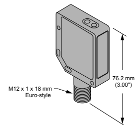
Figure 6. Quick-Disconnect Models
