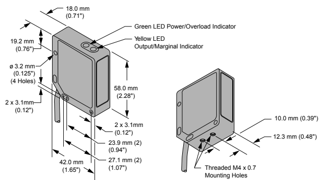
Figure 5. Cabled Models
