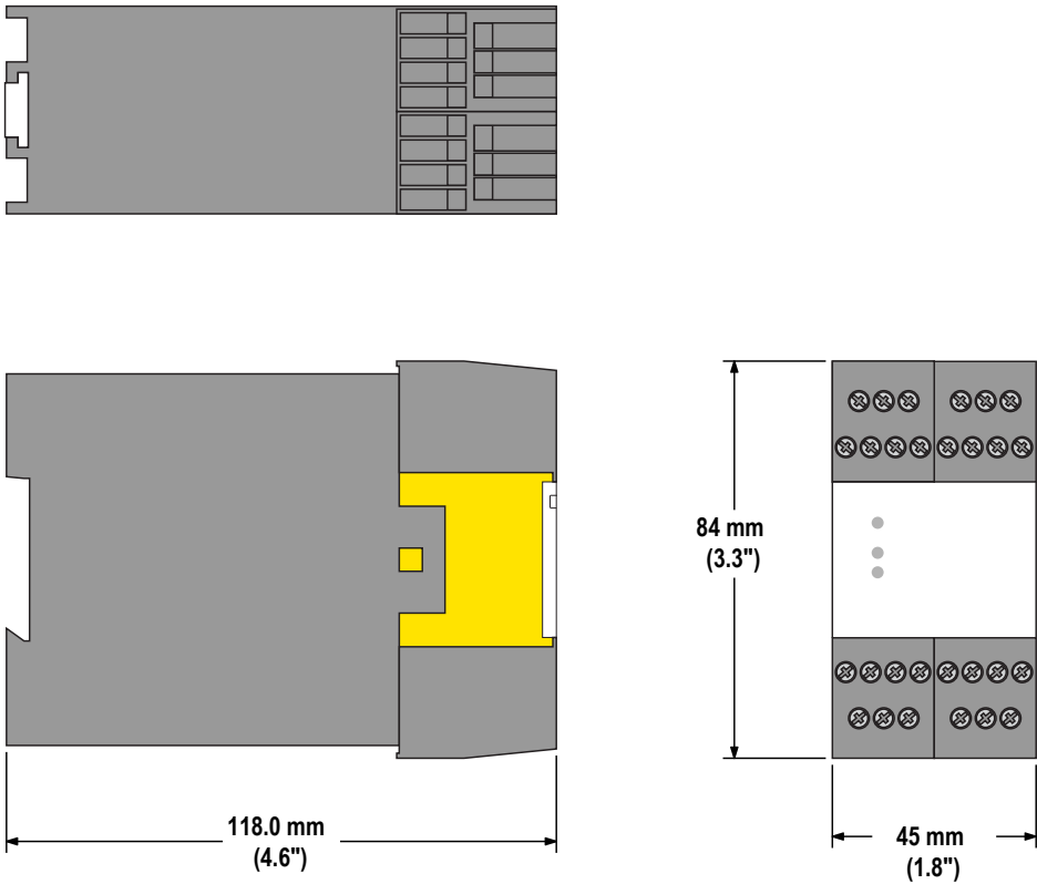
Dimensions—SSM-FM-11A20
