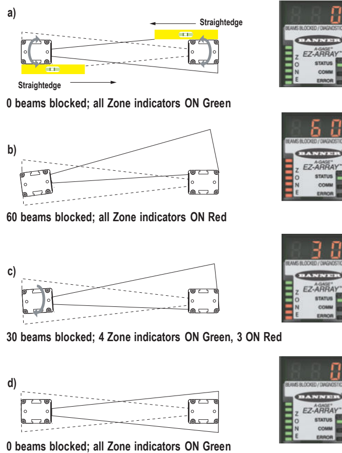
Figure 6. Optical alignment
