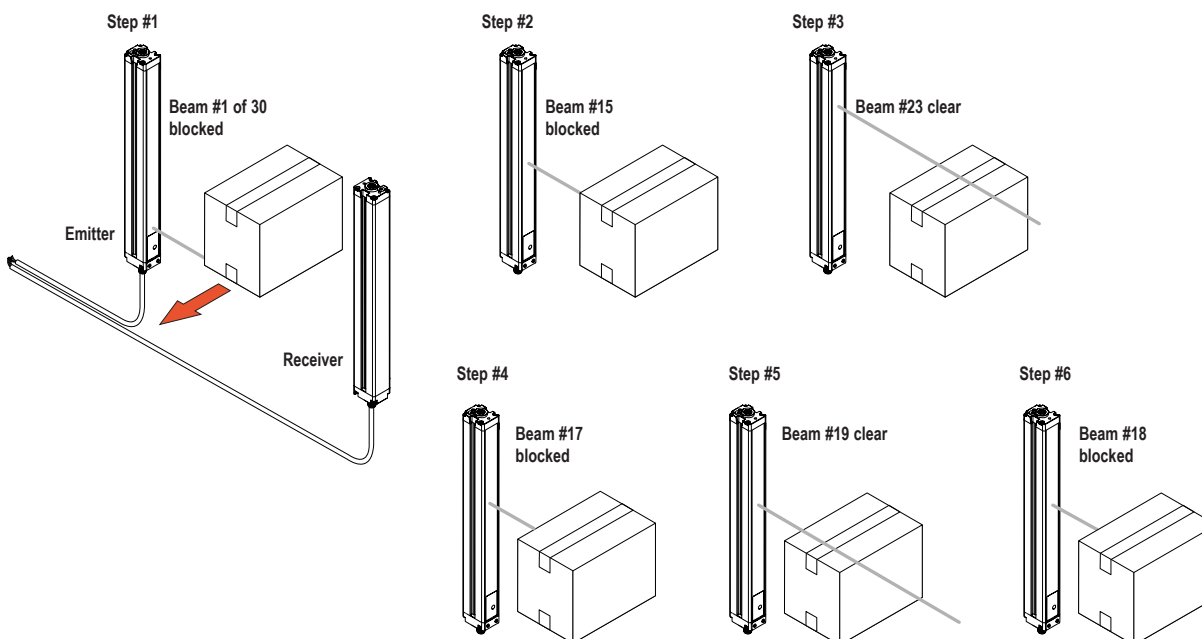
Figure 5. Double-edge scan
