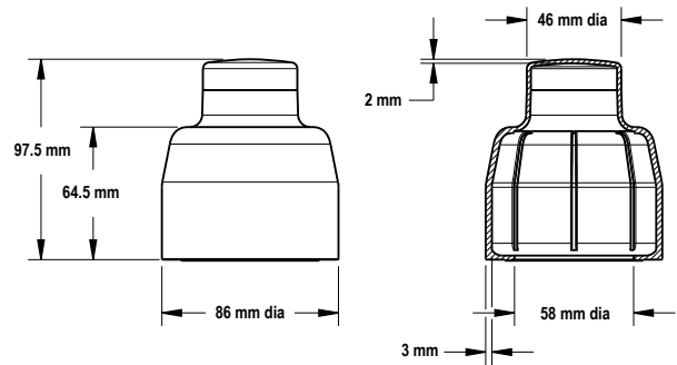
Washdown silicone cover SSA-EB1P-ECWC
