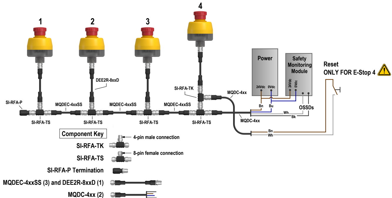
SSA-EB1PLx-0Dx E-Stops with ISD Series Connection
