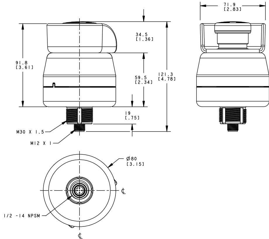
Dimensions for the SSA-EB1 PLXXS1 12ECQ8 E-stop button with shroud
