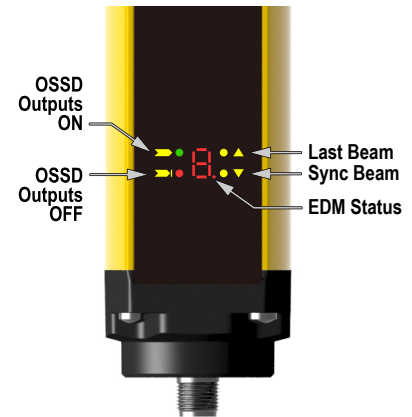
Status Indicators—Receiver
