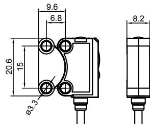
Sensor with Bracket (SMBVS8DT)
