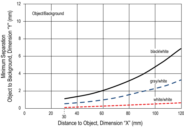
Minimum separation between object and background (Background Suppression Mode) for AF120 models
