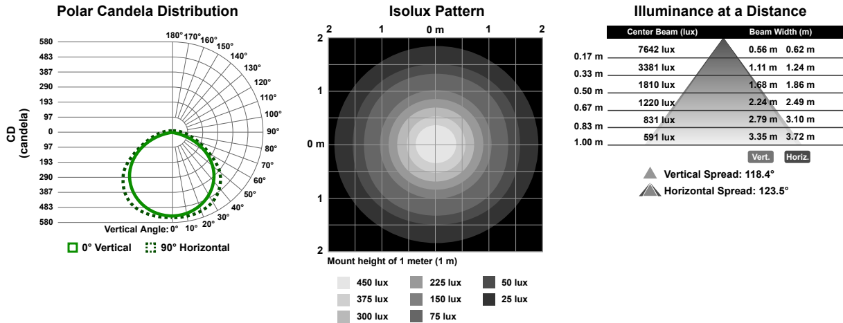
Figure 7. 710 mm Models
