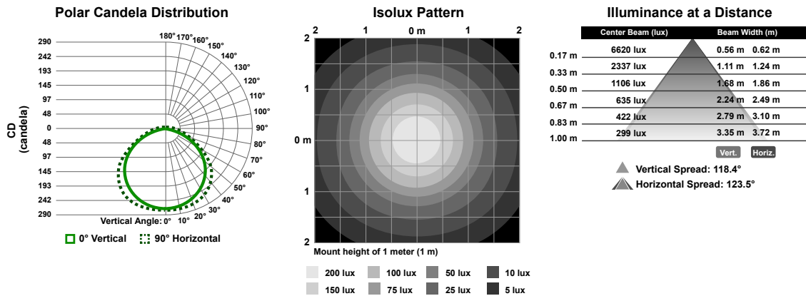
Figure 5. 430 mm Models
