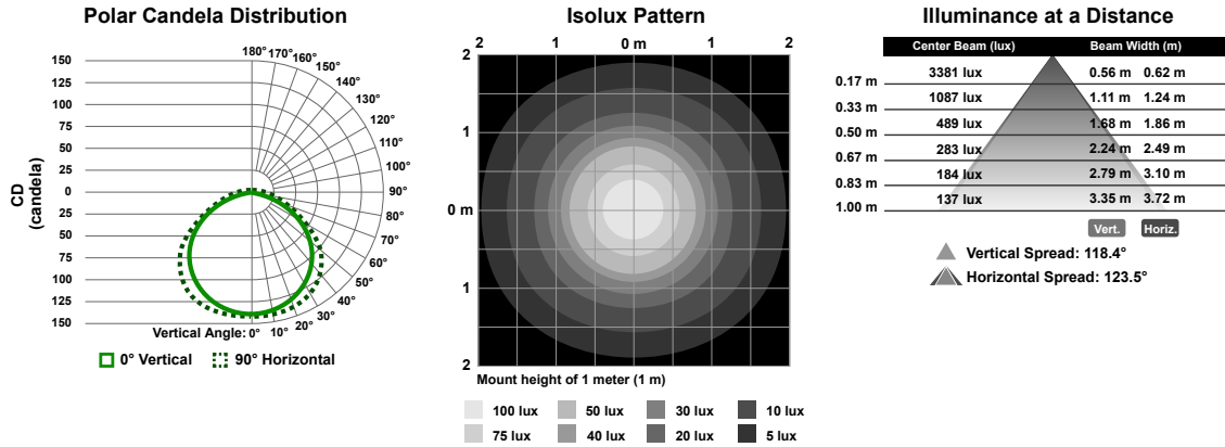
Figure 4. 285 mm Models
