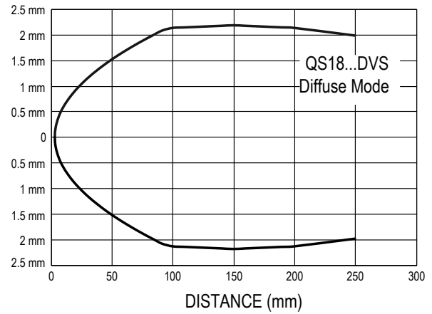
Beam Pattern
