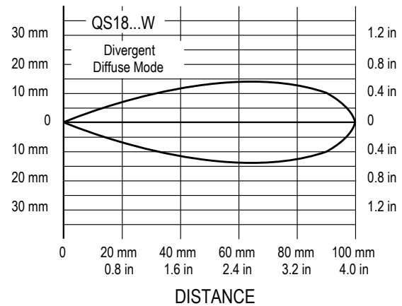
Beam Pattern
