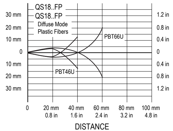
Beam Pattern
