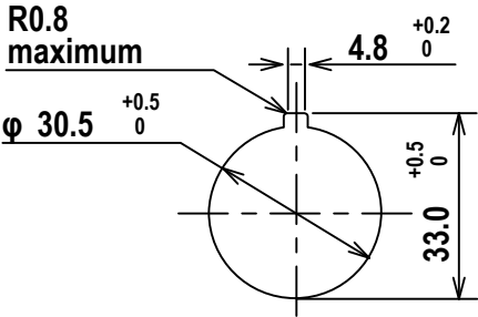
Notch dimensions
