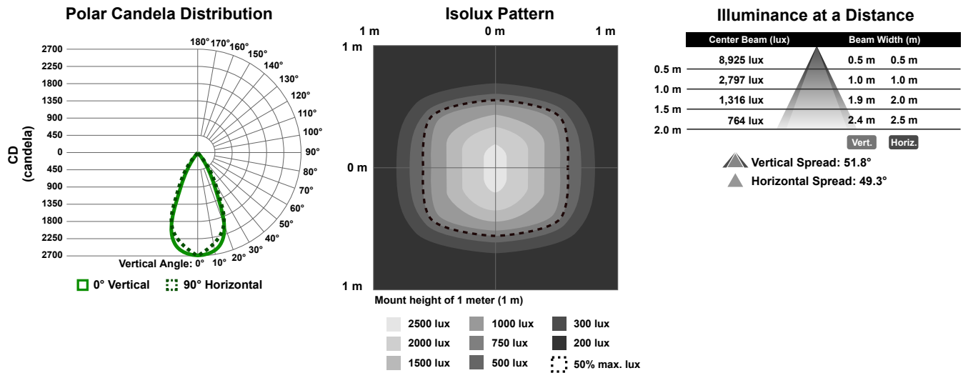
Figure 2. 640 mm Models
