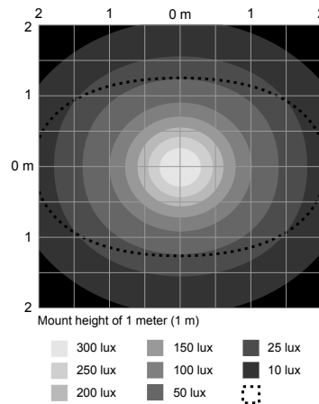
Isolux Pattern
