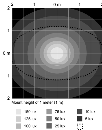
Isolux Pattern
