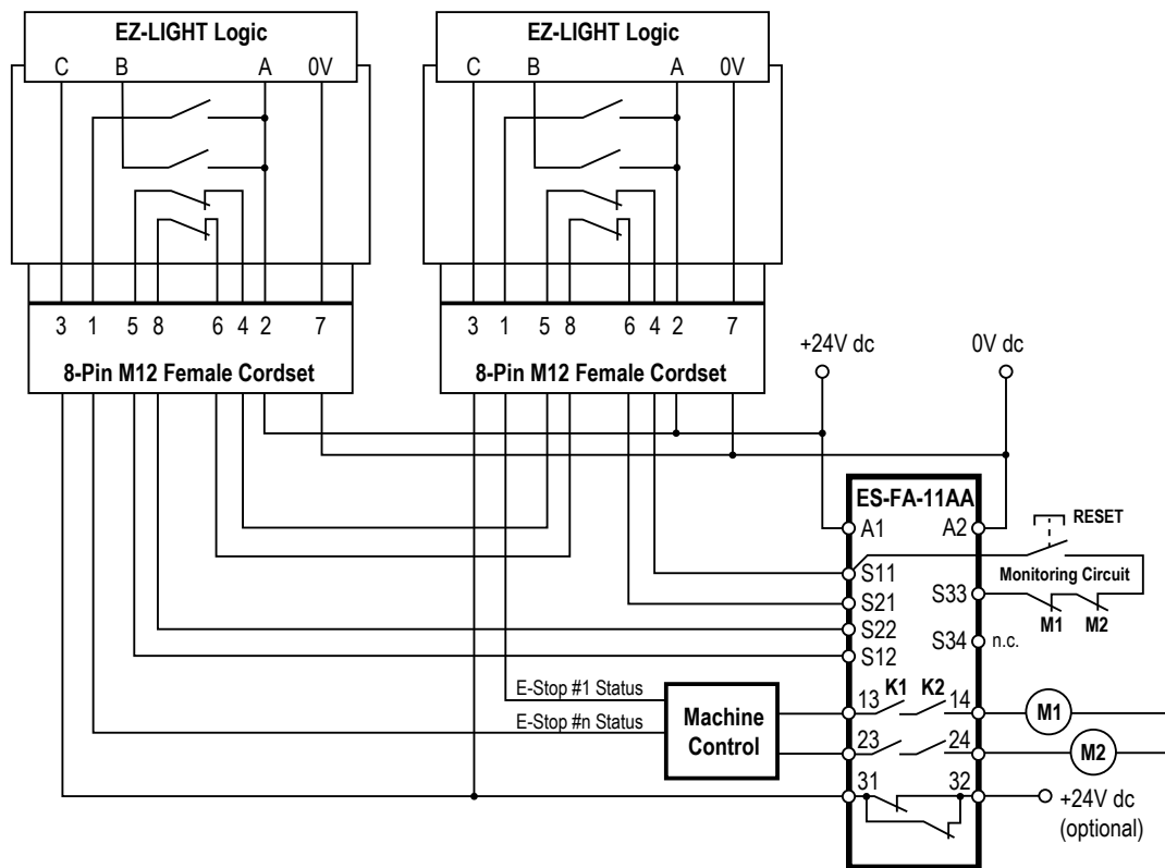
Illuminated models - example hookup
