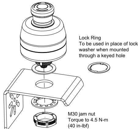
Mounting the E-stop
