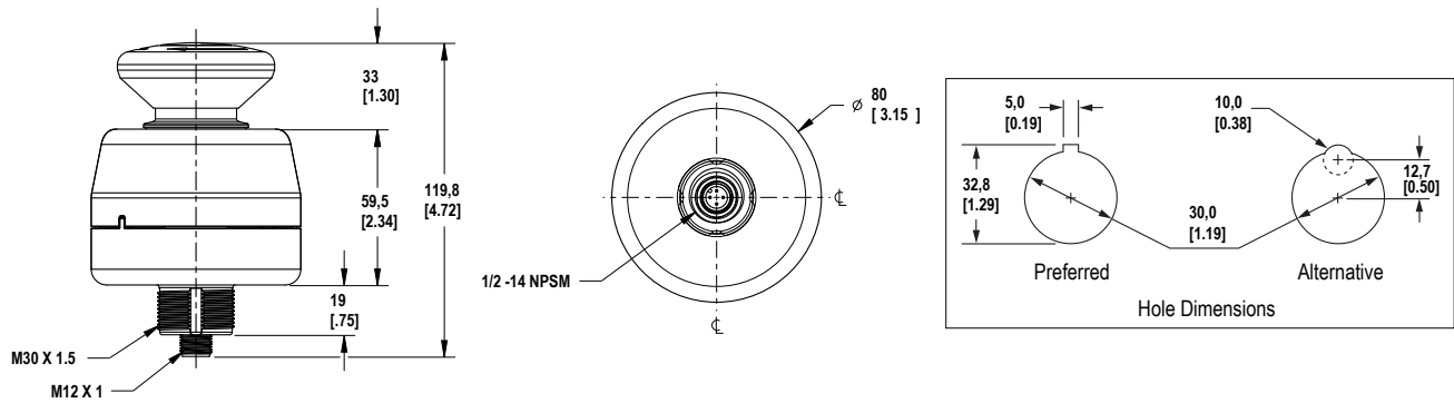
Large 60 mm Pushbutton
