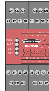
Indicator and Terminal Locations
