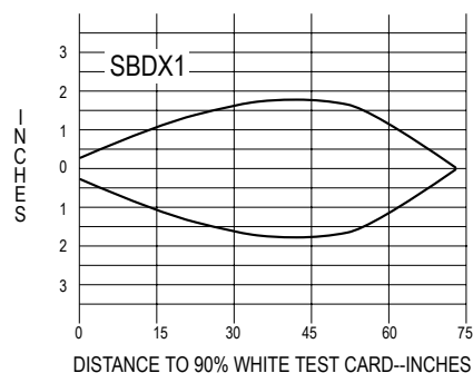
Figure 10. Beam Pattern - SBDX1MD
