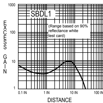
Figure 5. Excess Gain - SBDL1
