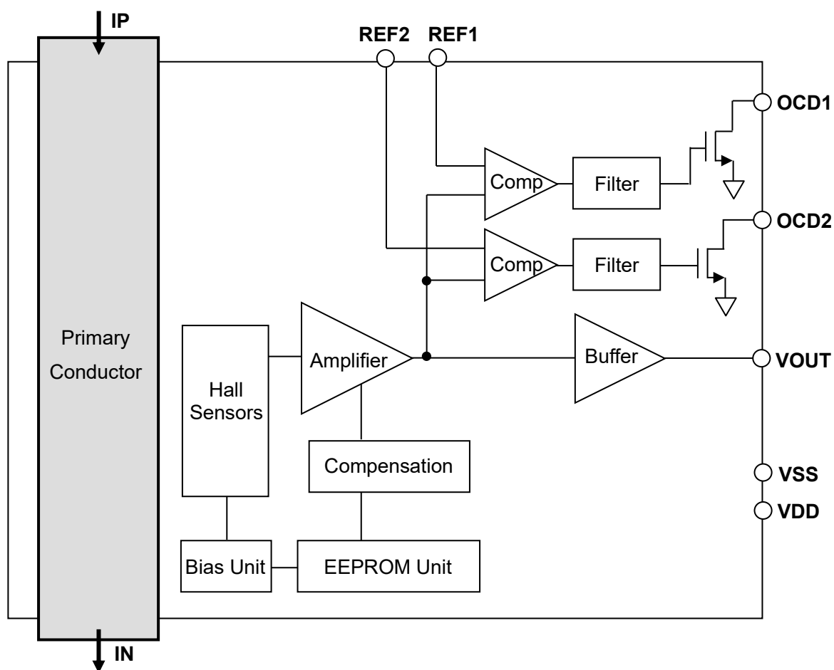
Figure 1. Block diagram of CZ-3AG5
