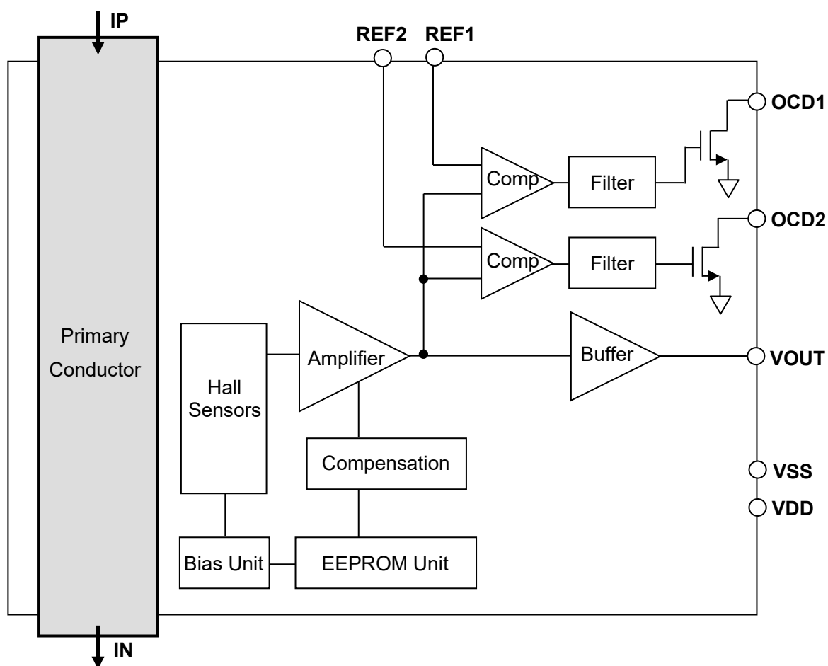
Figure 1. Block diagram of CZ-3AG4
