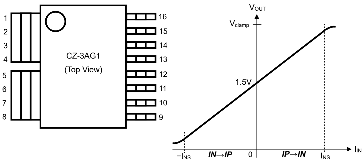
Figure 2. Pin configurations and typical output characteristics of CZ-3AG1
