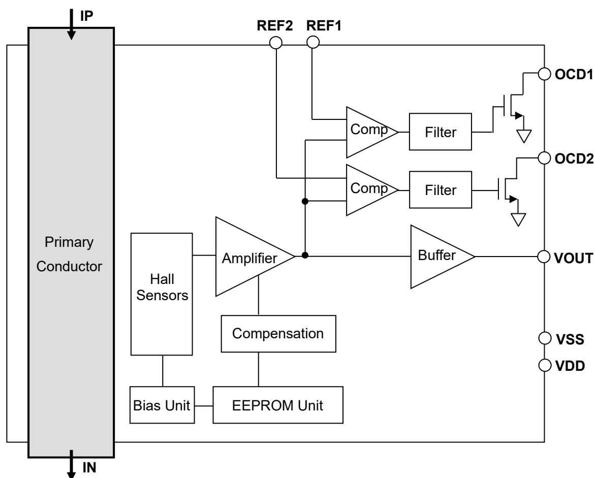
Figure 1. Block diagram of CZ-3AG1
