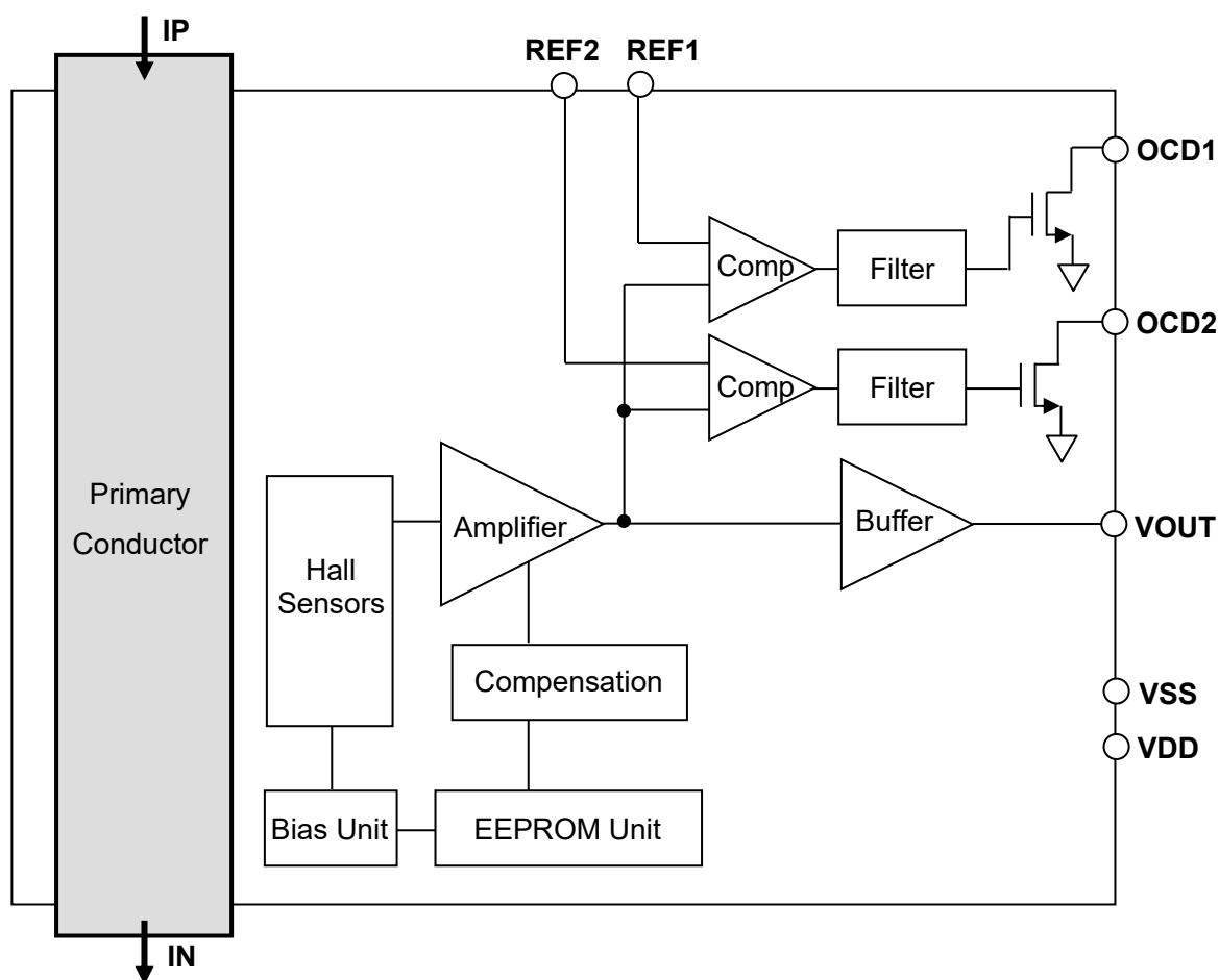
Figure 1. Block diagram of CZ-3A07
