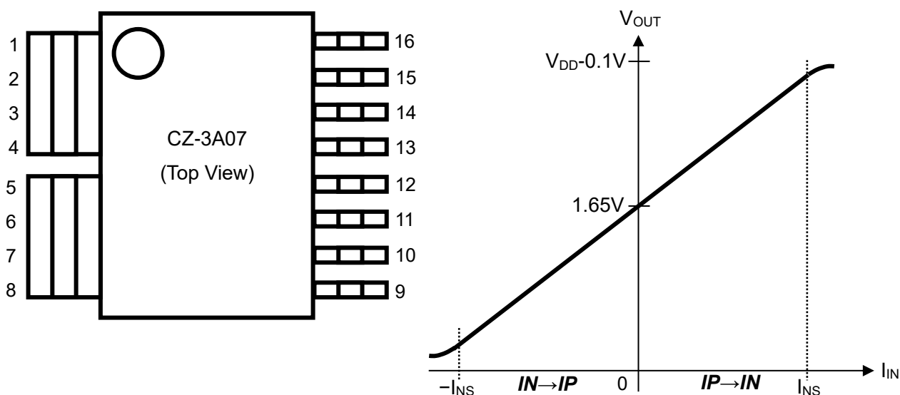
Figure 2. Pin configurations and typical output characteristics of CZ-3A07
