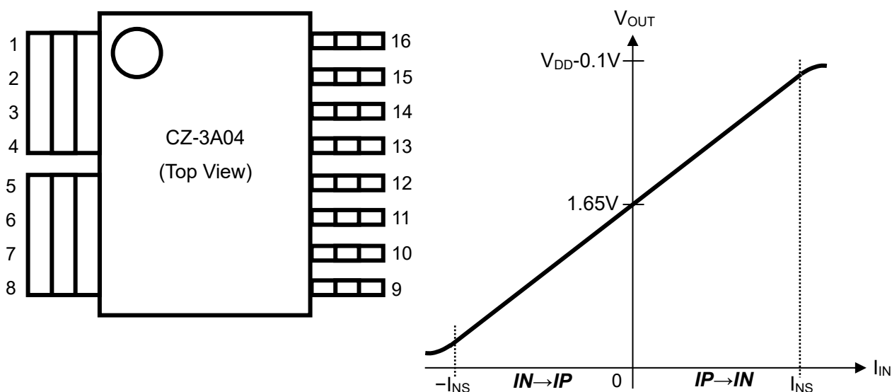
Figure 2. Pin configurations and typical output characteristics of CZ-3A04
