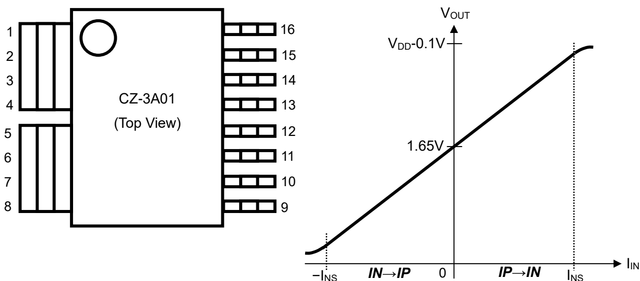
Figure 2. Pin configurations and typical output characteristics of CZ-3A01
