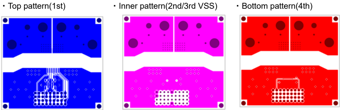
Figure 7. Board layout for measuring thermal resistance of CZ-3701
