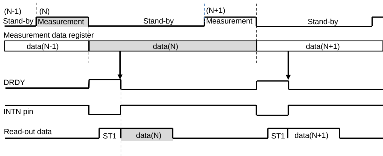
Figure 11.3 Read-out Procedure
