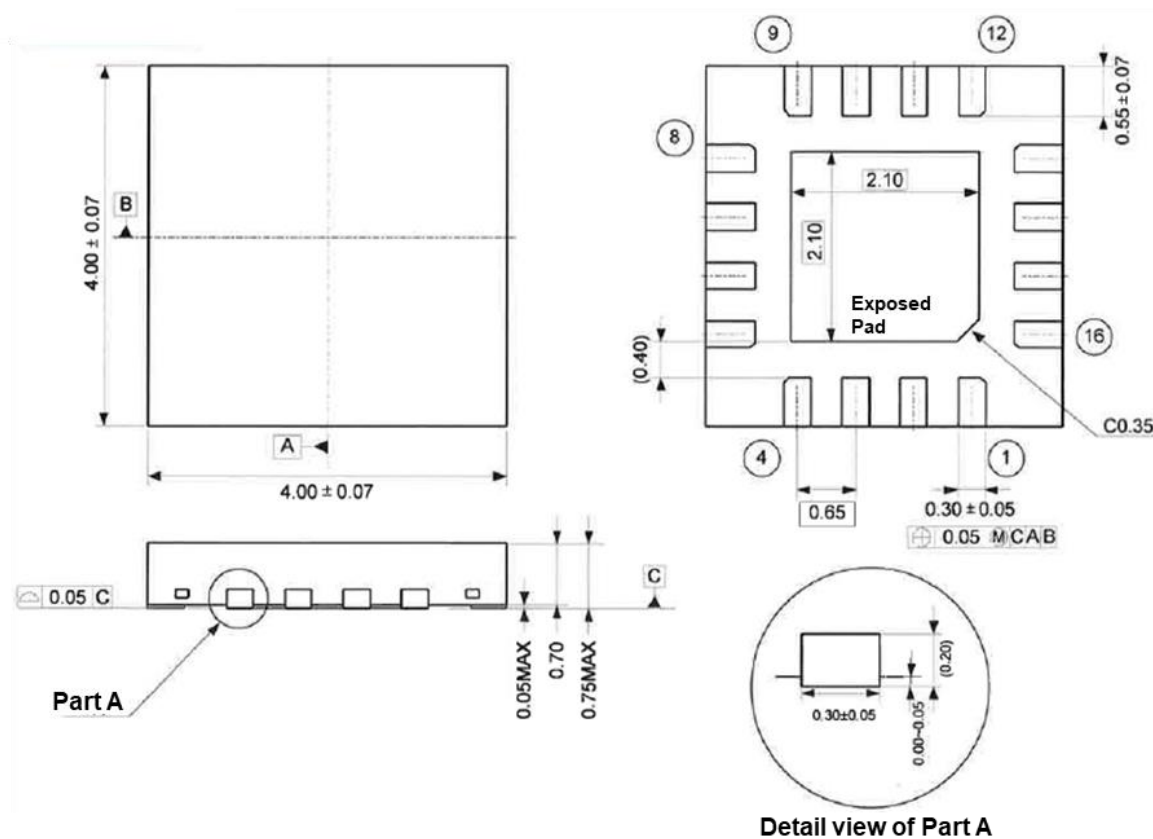
Figure 15.1 Outline Dimensions
