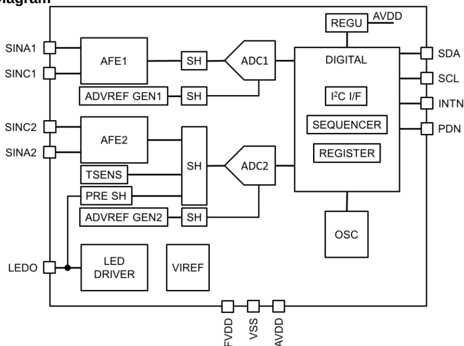
Figure 5.1 Block Diagram
