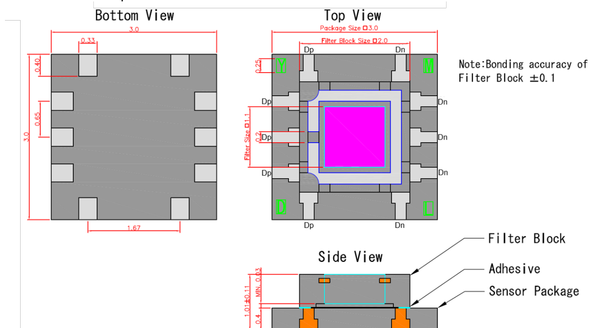
Figure 11.1 Outline Dimensions
