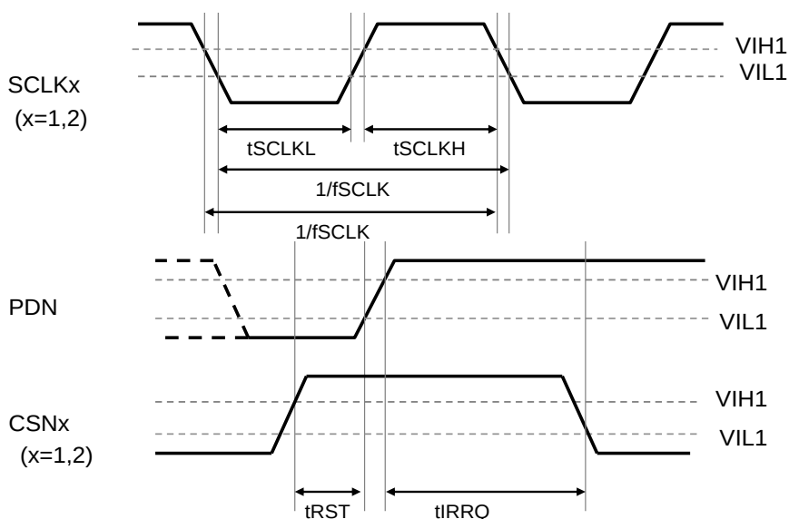
Figure 11. SPI Interface Timing 1
