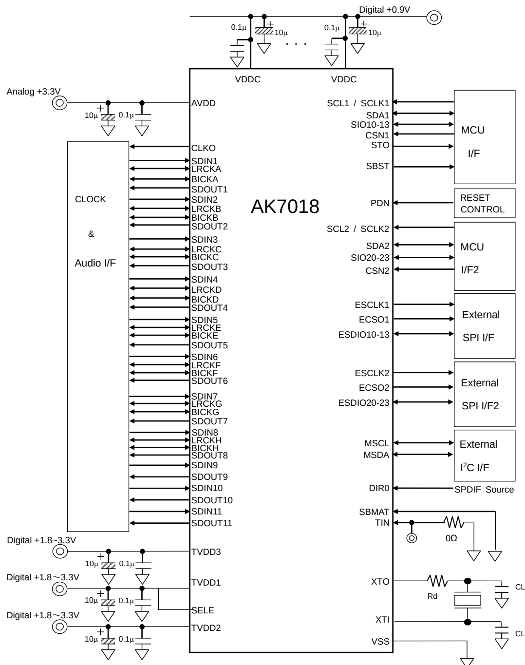
Figure 18. Connection Example
