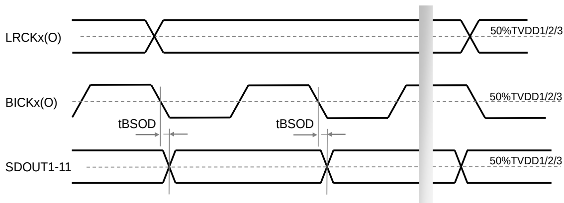
Figure 10. Serial Interface Output Timing in Master Mode
