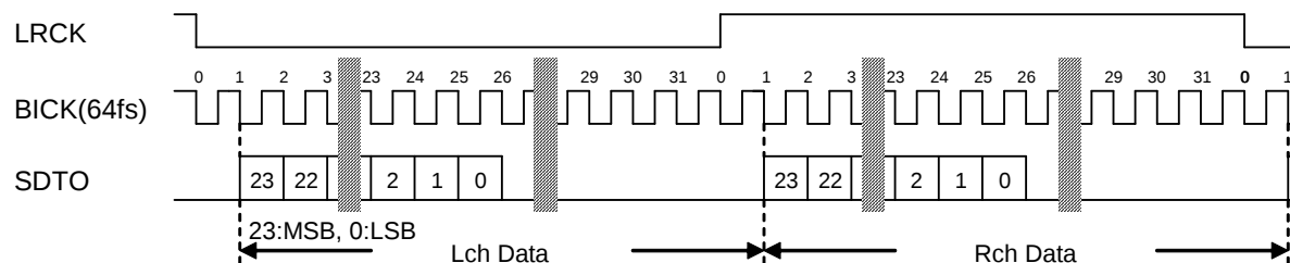
Figure 9. Mode 1, 3, 5, 7 Timing (Normal mode, I 2 S Compatible)
