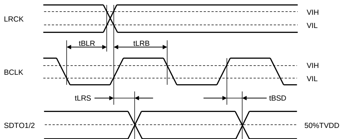
Figure 5. Audio Interface Timing (Normal &amp; Slave Mode: BCKP bit = "1")
