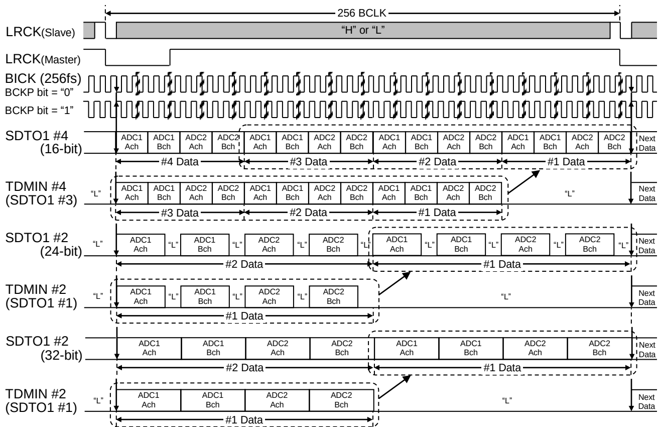
Figure 24. Mode 16/20 Timing (TDM256 mode, I 2 S Compatible)
