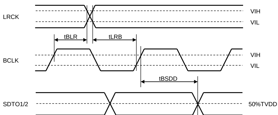
Figure 6. Audio Interface Timing (PCM &amp; Slave Mode: BCKP bit = "0")
