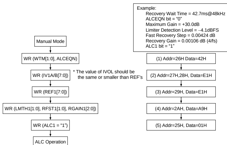
Figure 41. ALC Operation Setting Sequence
