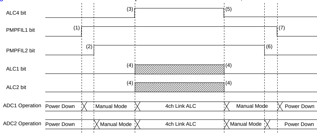
Figure 43. 4ch Link ALC Mode Sequence (ALC4 bit = "1")
