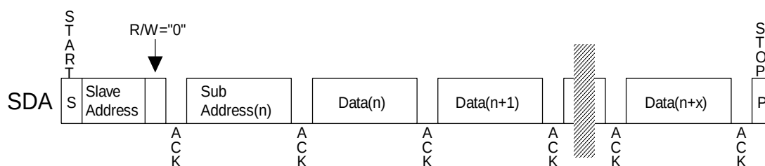
Figure 47. Data Transfer Sequence at I 2 C Bus Mode
