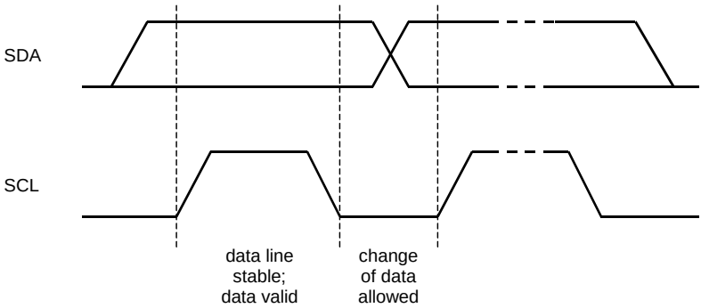
Figure 55. Bit Transfer (I 2 C Bus)
