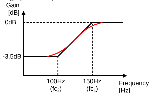
Figure 40. ALCEQ Frequency Response (fs = 48kHz)
