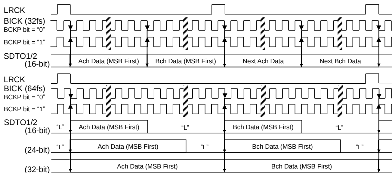
Figure 20. Mode 2/6 Timing (Normal mode, PCM Short Frame)
