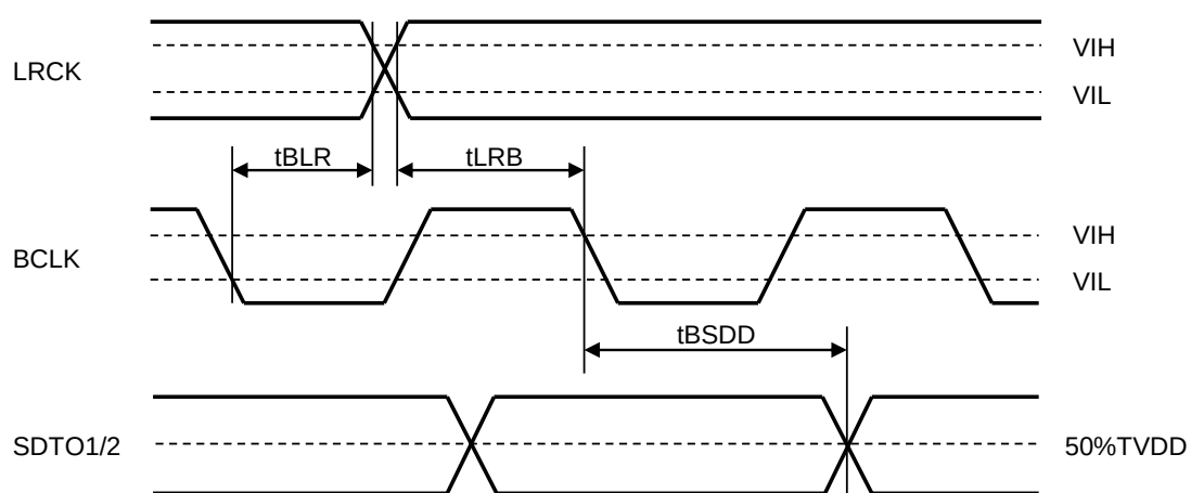
Figure 7. Audio Interface Timing (PCM &amp; Slave Mode: BCKP bit = "1")
