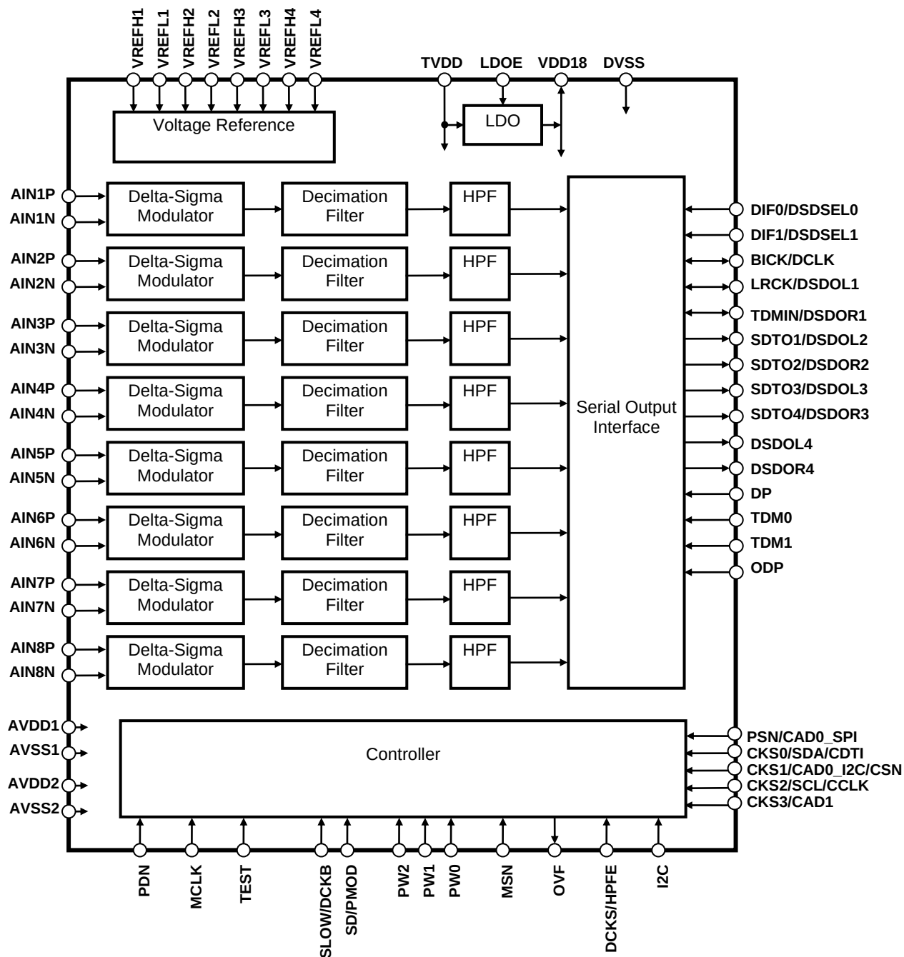
Figure 1. Block Diagram
