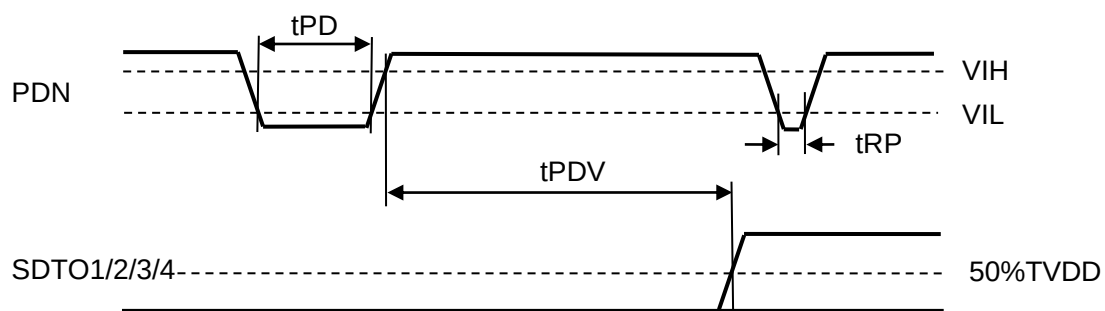
Figure 28. Power-down &amp; Reset Timing
