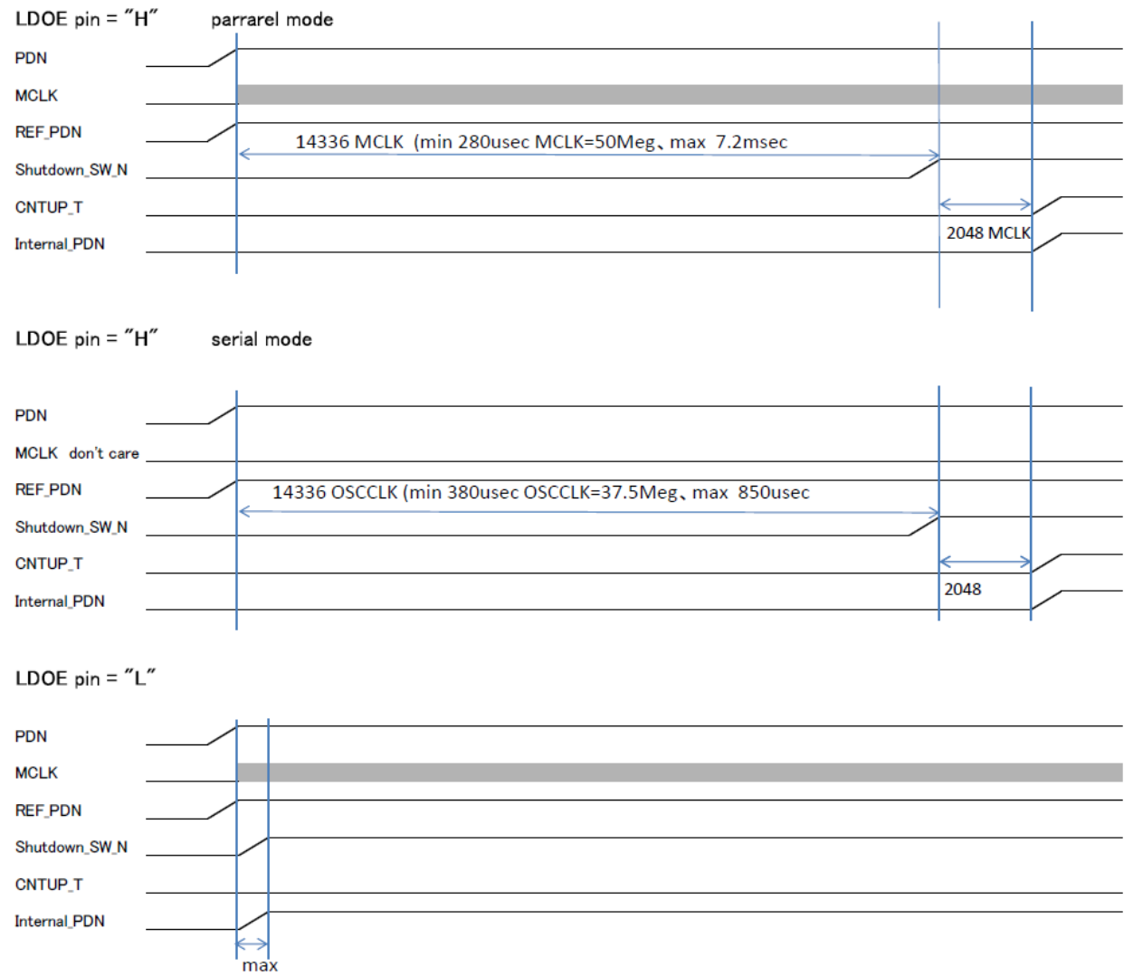
Figure 60. Internal PDN Release Sequence
