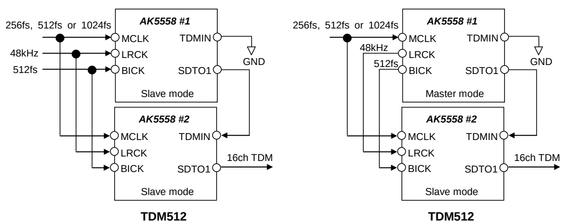
Figure 29. Cascade Connection
