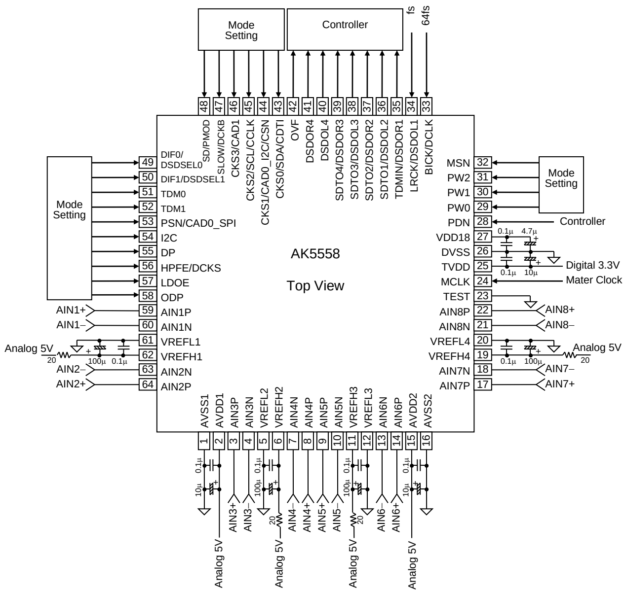
Figure 75. Typical Connection Diagram
