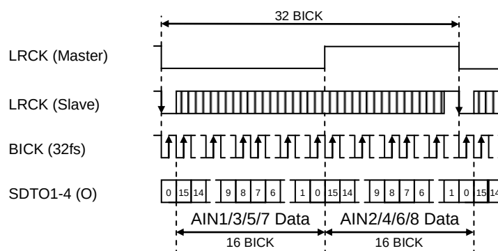
Figure 35. Mode 9/17 Timing (Normal Output, OCT/HEX Speed Mode, I²S Compatible, 16-bit)
