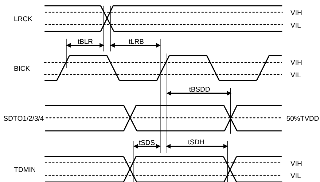
Figure 21. Audio Interface Timing (TDM &amp; Slave Mode)
