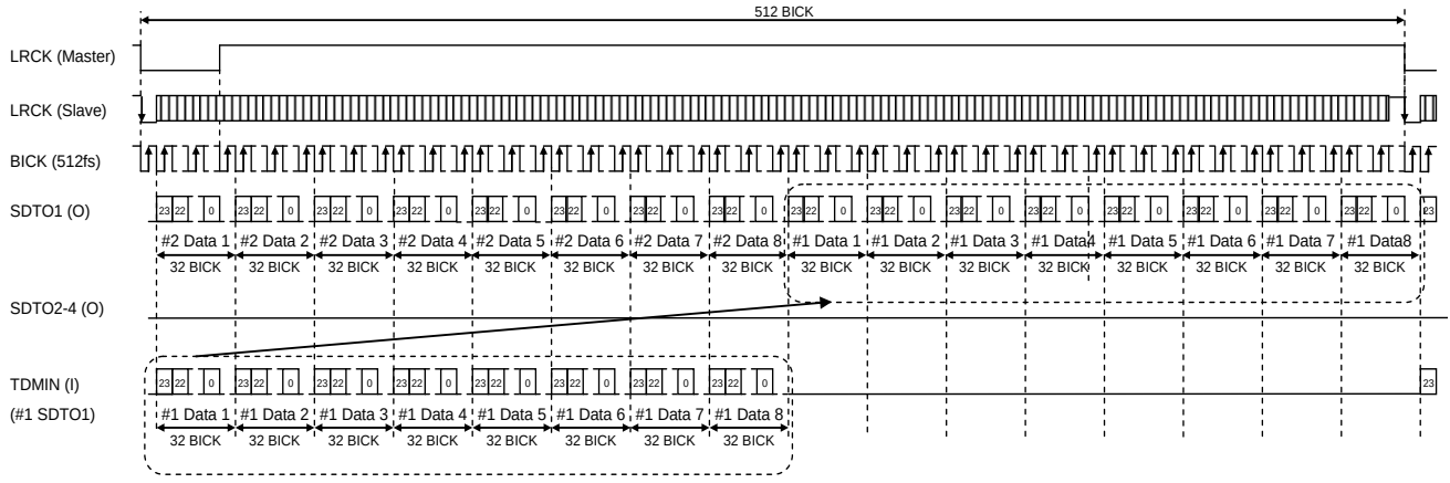
Figure 51. Mode 41/45 Timing (TDM512 Mode, I²S Compatible, 24-bit)
