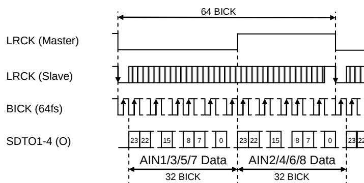
Figure 39. Mode 13/21 Timing (Normal Output, OCT/HEX Speed Mode, I²S Compatible, 24-bit)
