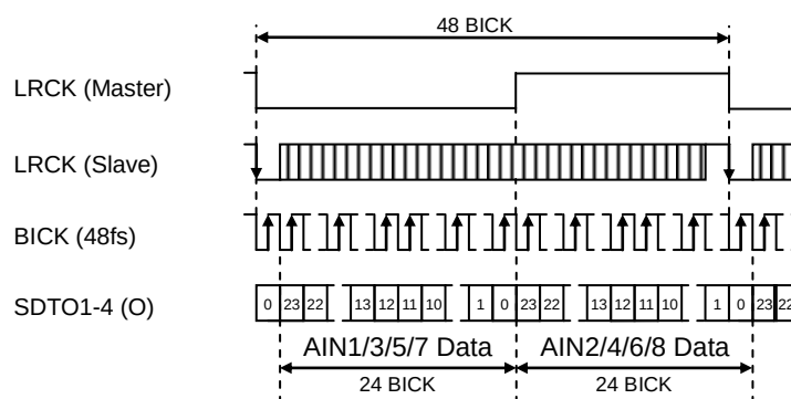
Figure 37. Mode 11/19 Timing (Normal Output, OCT/HEX Speed Mode, I²S Compatible, 24-bit)
