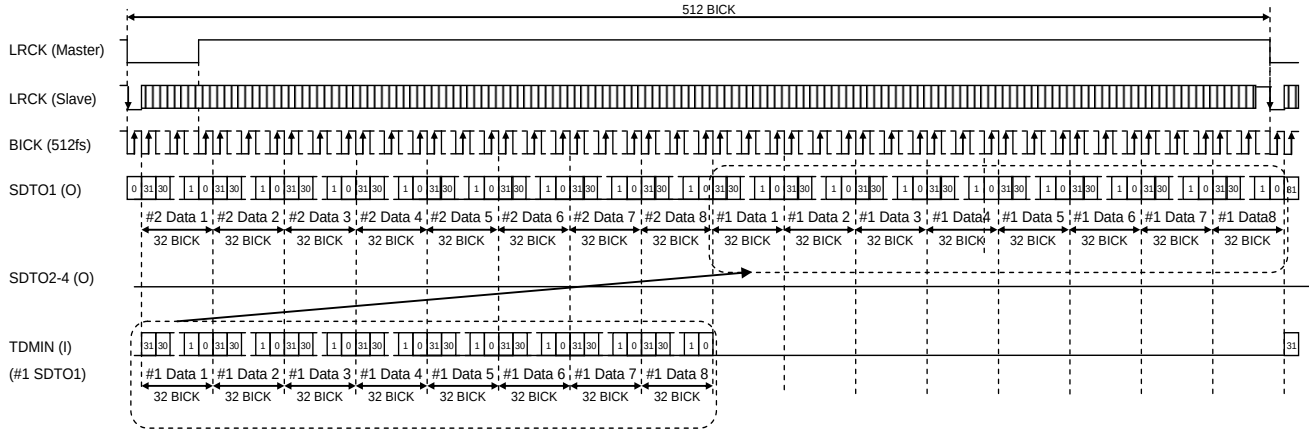
Figure 53. Mode 43/47 Timing (TDM512 Mode, I²S Compatible, 32-bit)
