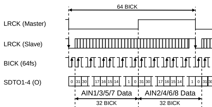
Figure 41. Mode 15/23 Timing (Normal Output, OCT/HEX Speed Mode, I²S Compatible, 32-bit)
