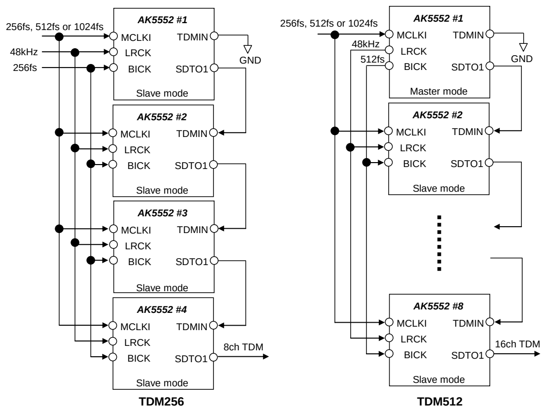
Figure 29. Cascade Connection
