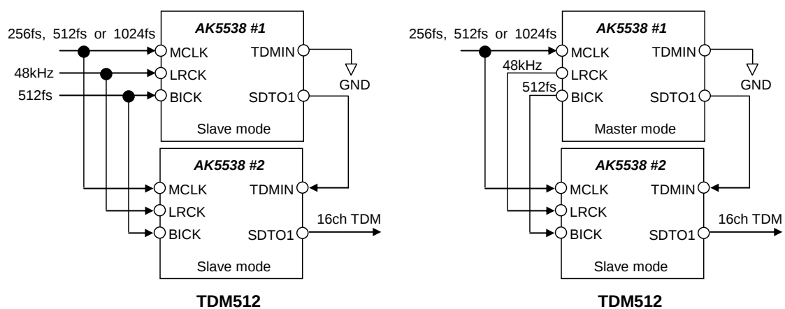
Figure 29. Cascade Connection
