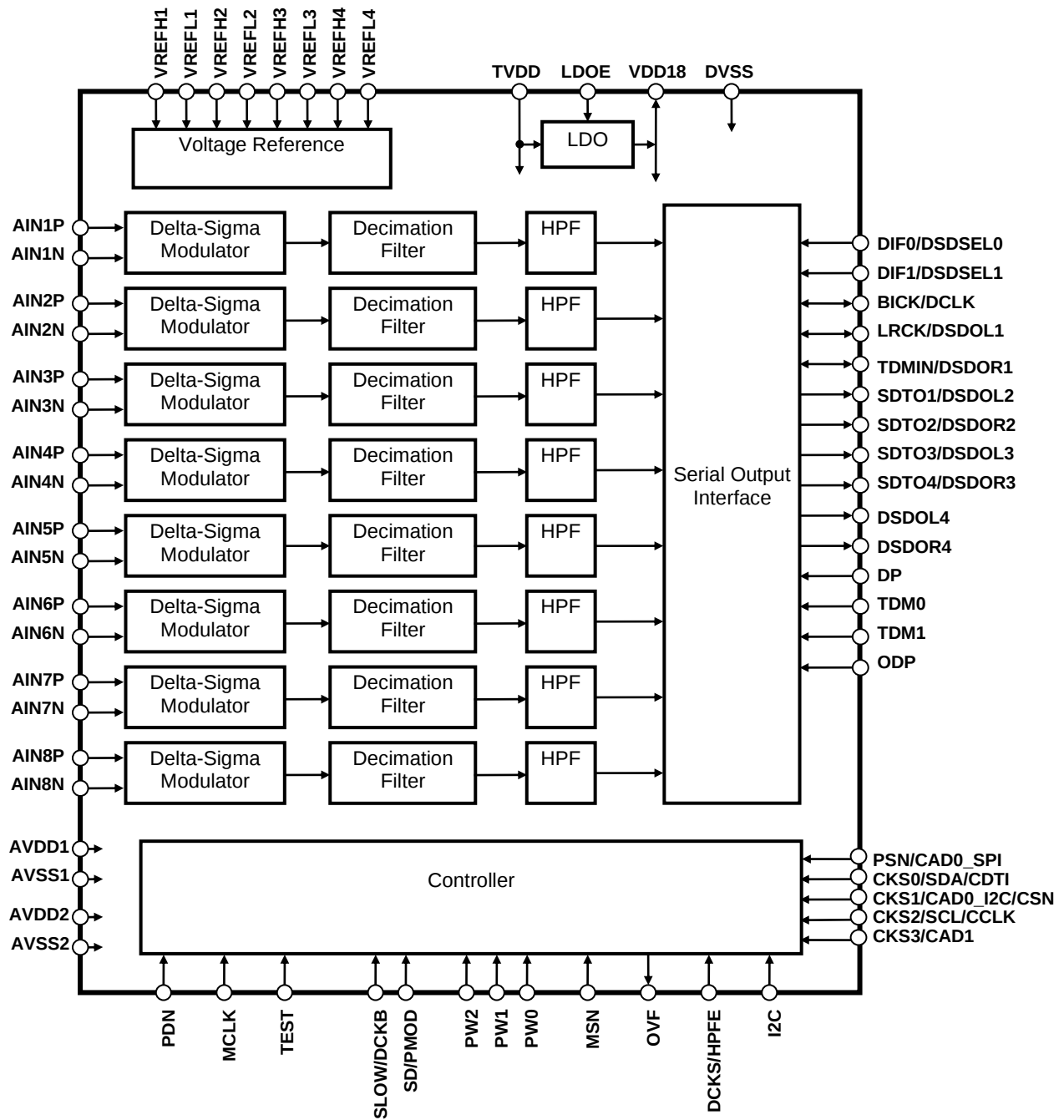
Figure 1. Block Diagram
