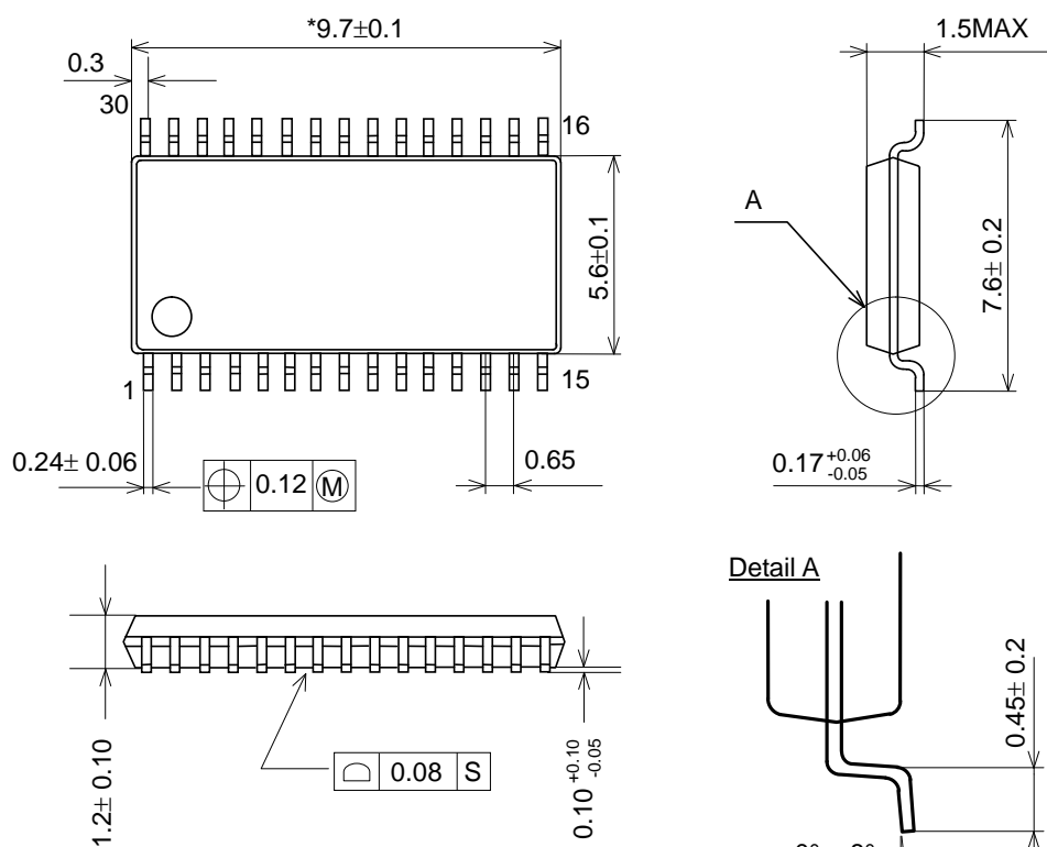
30pin VSOP (Unit: mm)
