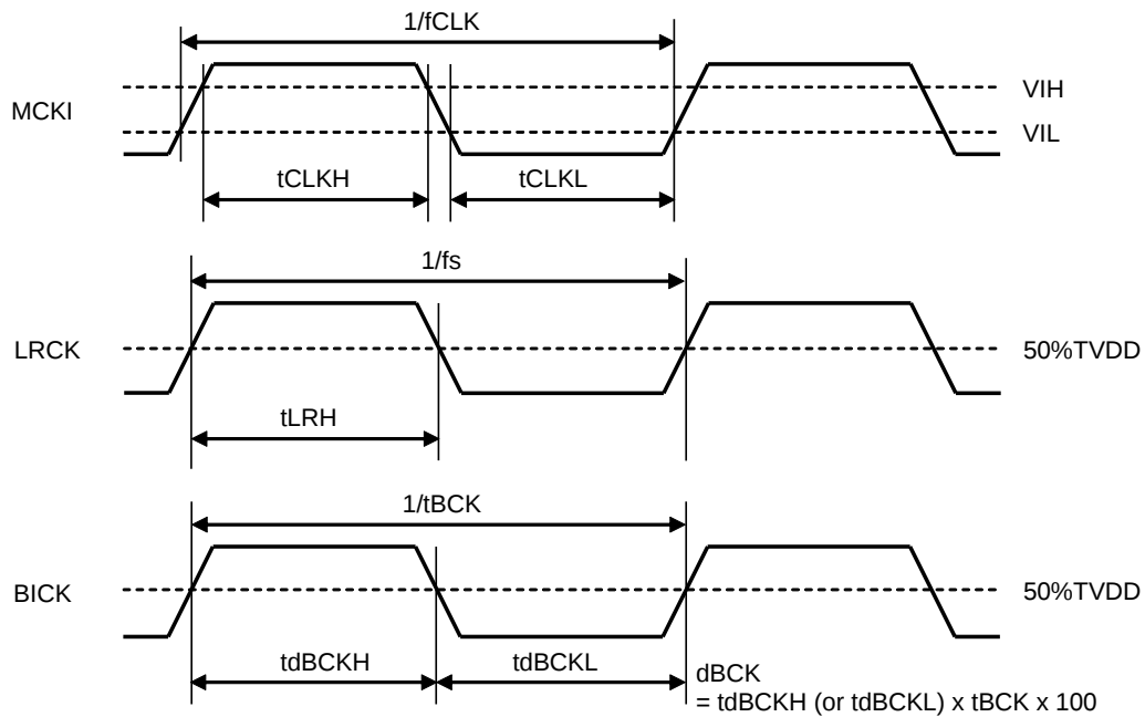
Figure 5. Clock Timing (Except TDM1-0 bits = "00" &amp; Master Mode)
