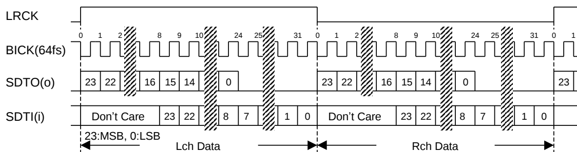
Figure 22. Mode 4/12 Timing
