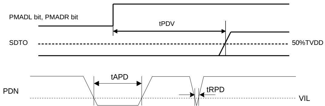
Figure 11. Power-down &amp; Reset Timing
