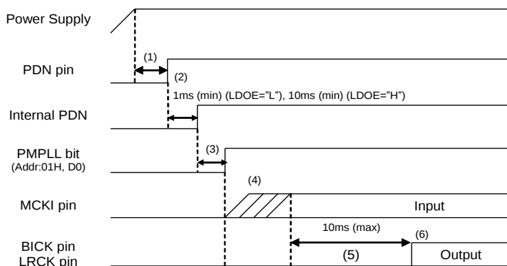
Figure 53. Clock Set Up Sequence (1)
