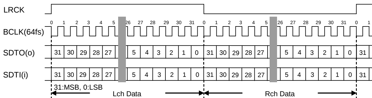
Figure 23. Mode 5/13 Timing
