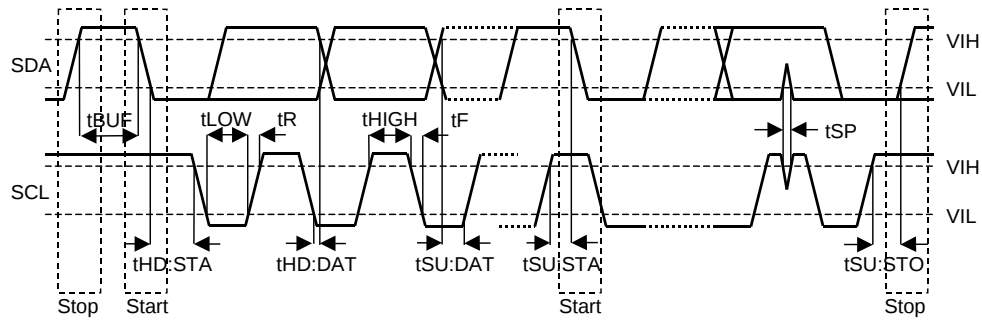
Figure 10. I²C Bus Mode Timing
