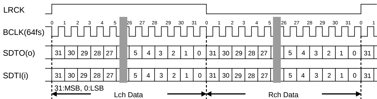
Figure 24. Mode 6/14 Timing
