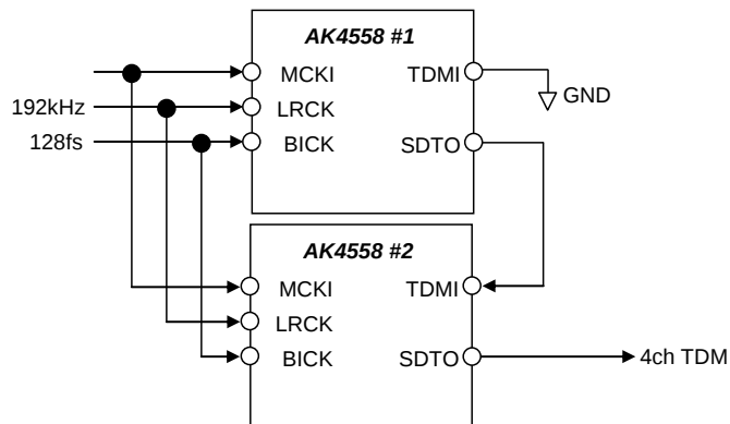
Figure 28. Cascade TDM128 Connection Diagram
