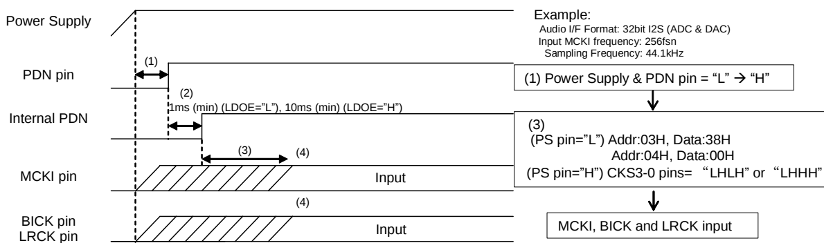
Figure 55. Clock Set Up Sequence (3)
