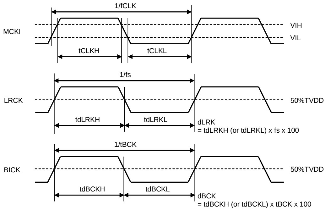
Figure 4. Clock Timing (TDM1-0 bits = "00" &amp; Master Mode)
