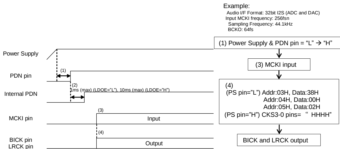
Figure 56. Clock Set Up Sequence (4)
