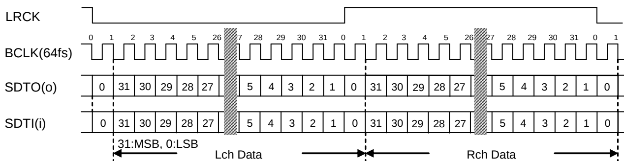
Figure 25. Mode 7/15 Timing
