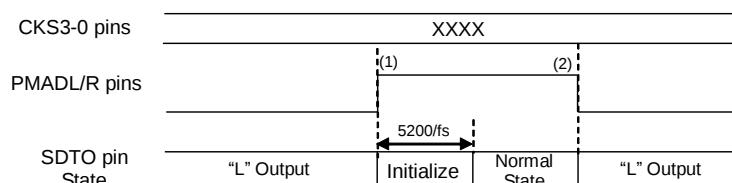
Figure 58. ADC Output Sequence (PS pin = “H”)
