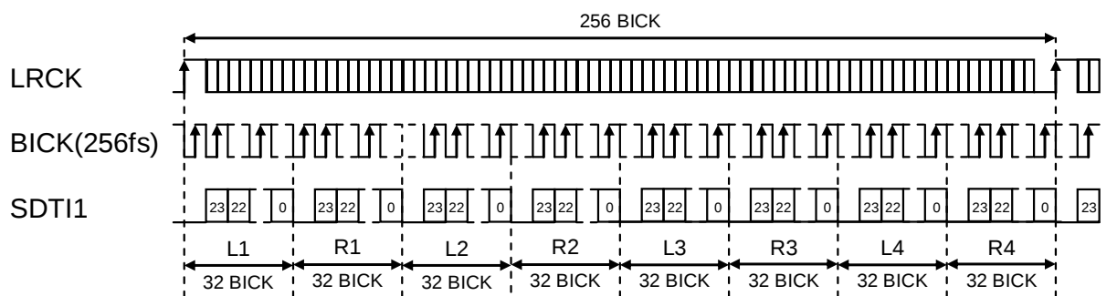
Figure 29. Mode 16 Timing
